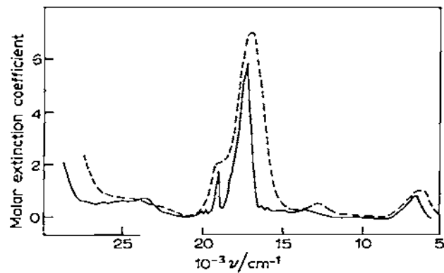
Fig. 7. Absorption spectrum of \text{CoCl}_2 : dashed, room temperature; solid trace, 20 K [81].
