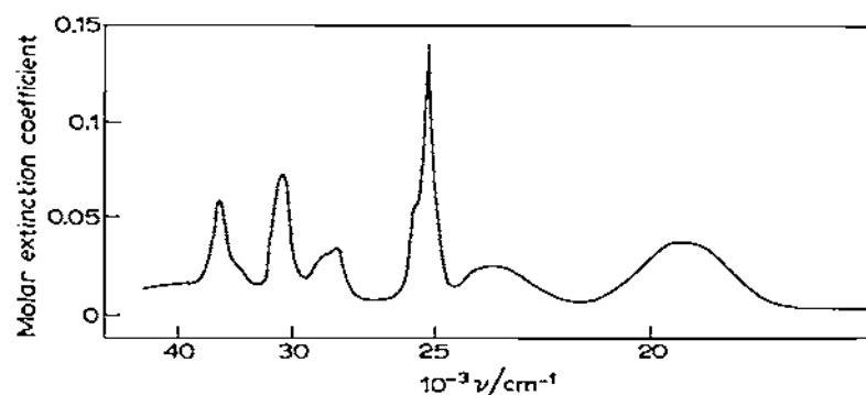
Fig. 4. Absorption spectrum of MnF 2 at room temperature [47].
