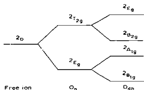
Fig. 3. Splitting of d^9 ^2D term in O_h and D_{4h} (elongated along z axis) ligand fields. (Not to scale). The ^2A_{1g} state may lie above the ^2B_{2g} or ^2E_g states depending on the degree of distortion.
